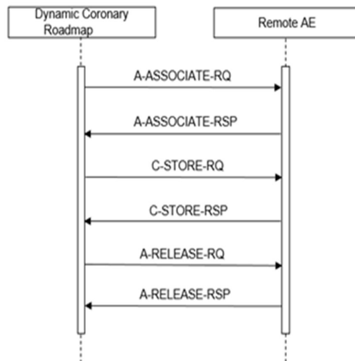
Figure 4 : Data Flow Diagram – Store Image – Storage as SCU
