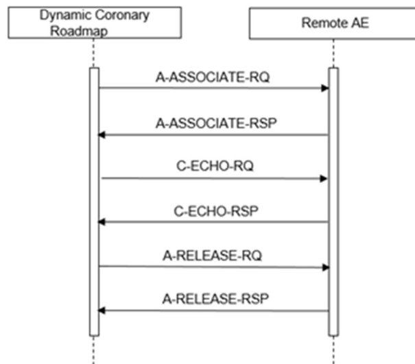
Figure 3: Data Flow Diagram – Verification as SCU
