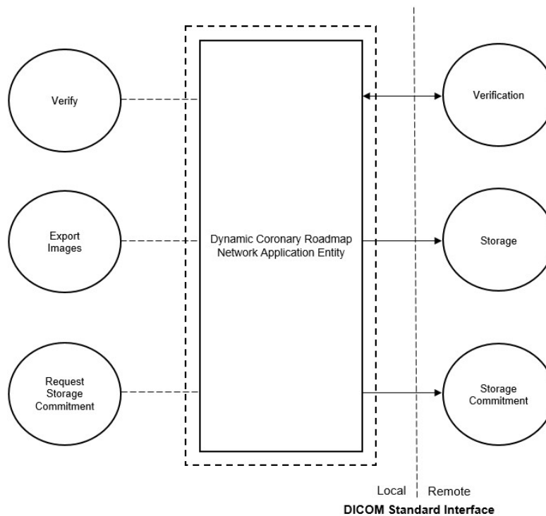
Figure 1: Application Data Flow Diagram
