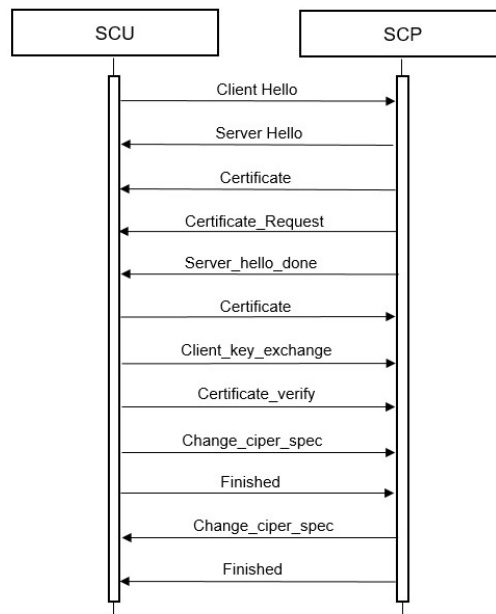
Figure 7 : Message flow of TLS handshake
