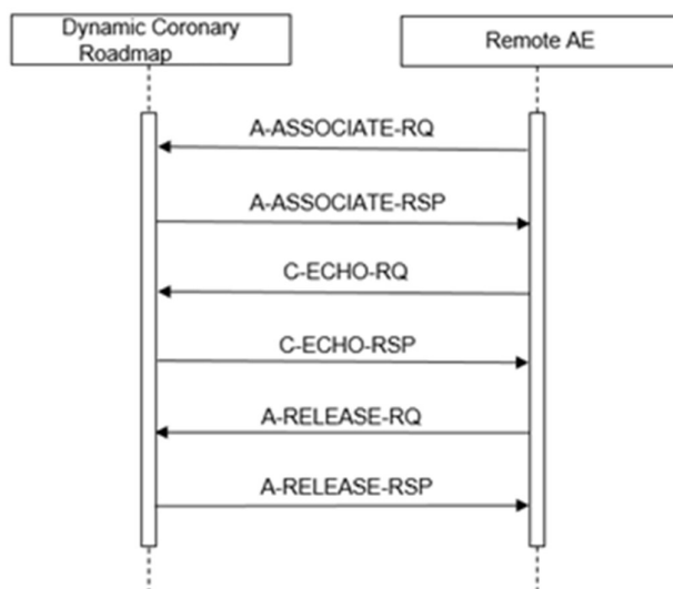
Figure 6: Verification as SCP
